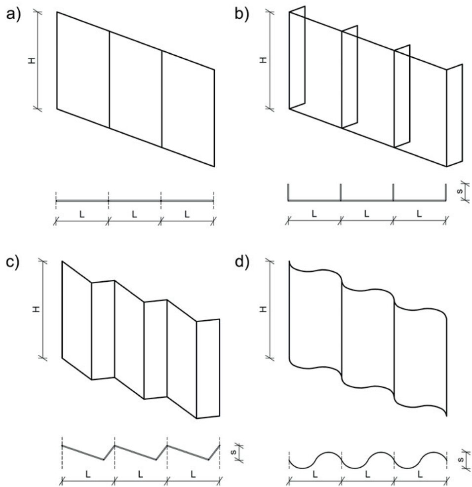
Ill. 3. Glass facades with structural glass: a) frameless system, b) facades with glass fins, c) glass folded plate system, d) facades with bent glass. Source: original work.
